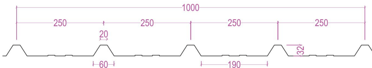
Profile YX-32/250-1000
