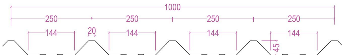
Profile YX-45/250-1000
